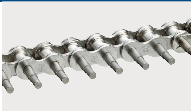
Marathon roller chain maintenance-free with offset and extended pins on one side
