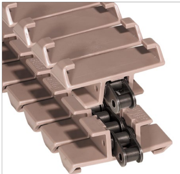
Photo shows 1873 TAB G TableTop Chain with Gripper Retainers molded in Low Friction (LF) material on Carbon Steel (S) base chain.
