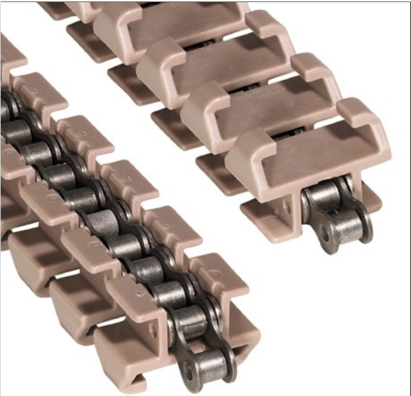
Photo shows 1843 TAB G TableTop Chain with Gripper Retainers molded in Low Friction (LF) material on Stainless Steel (SS) base chain.
