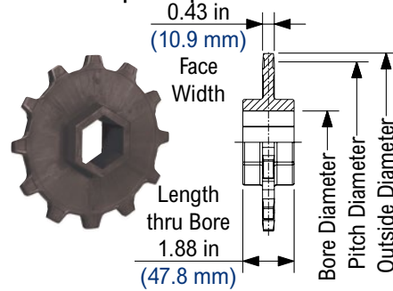
N1700 Thermoplastic Sprocket
