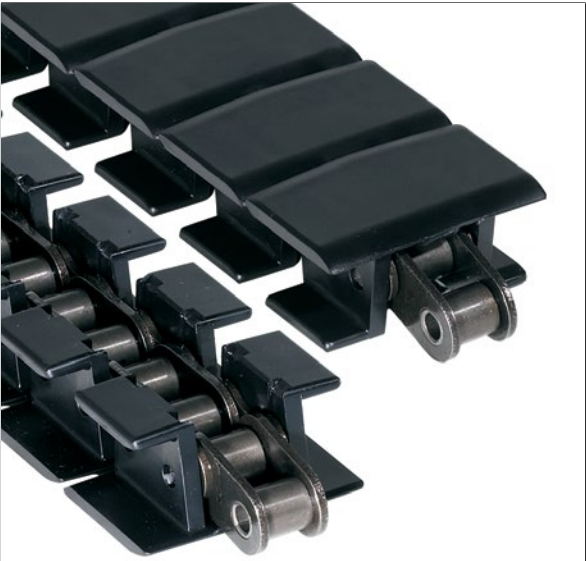
Photo shows 1863 TAB TableTop Chain with top plates molded in Black Wear Resistant (BWR) material on Carbon Steel (S) base chain.
