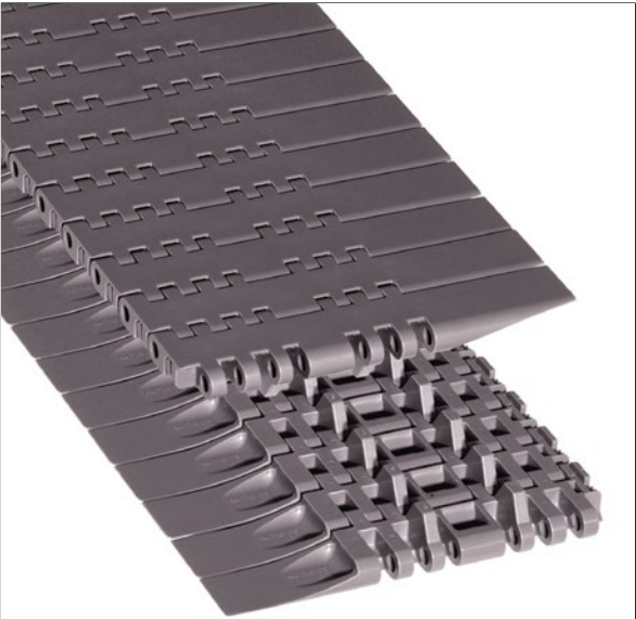
Photo shows 7705 MatTop Chain with DynamicTransfer System (DTS) and Positrack (PT) Tracking Guides molded in High Performance (HP) material.
