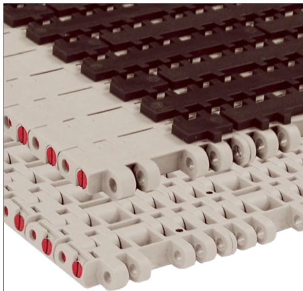
Photo shows 7705 RubberTop MatTop Chain molded in High Temperature Friction Top (HTF) material.
