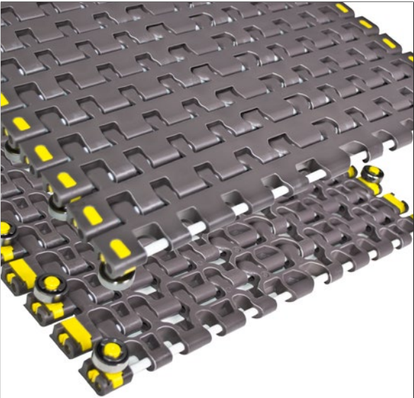
Photo shows 7956 B MatTop Chain with roller bearing attachment molded in High Performance (HP) material.
