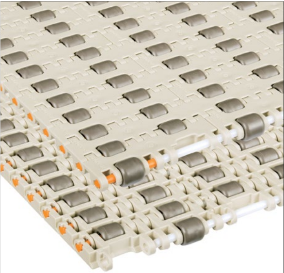
Photo shows 8503 MatTop Chain molded in High Temperature material.
