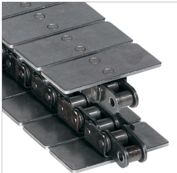
Photo shows 1864 TableTop Chain with Carbon Steel (S) top plates on Carbon Steel (S) base chain.
