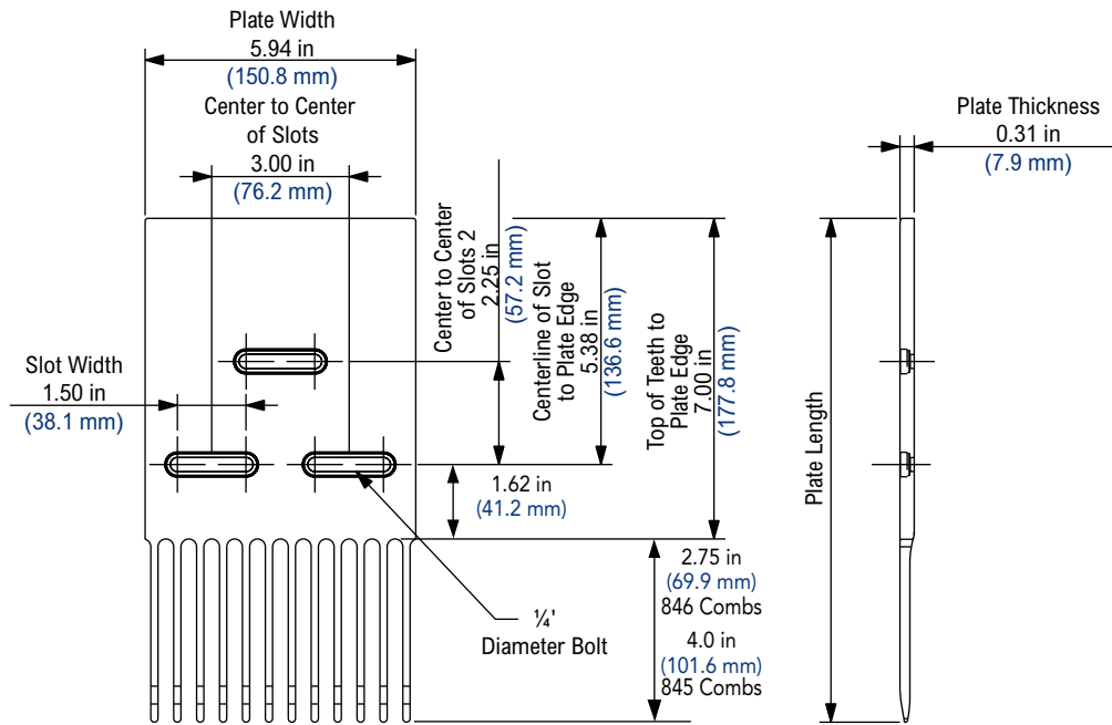
4707/5997/Fortex Retrofit Transfer Comb Kit
