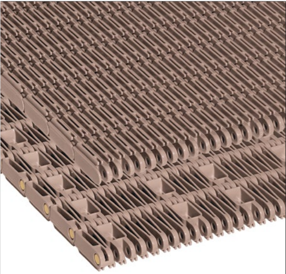
Photo shows 5997 MatTop Chain molded in High Temperature (HT) material.
