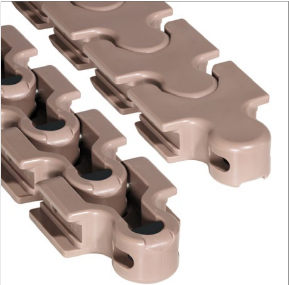
Photo shows 2550 TAB TableTop Chain molded in Low Friction (LF) material.
