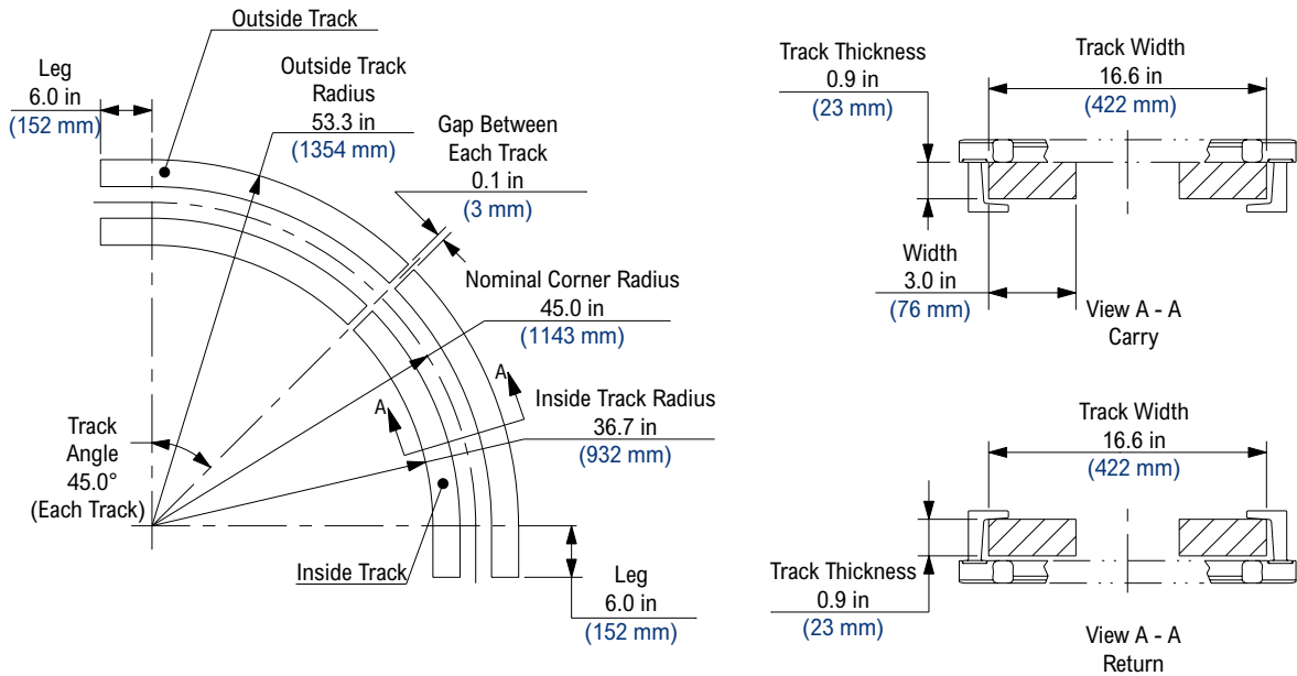
Corner Track (Four Piece)
