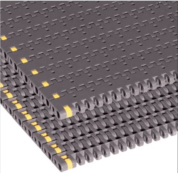
Photo shows 8505 V MatTop Chain with Vacuum Holes molded in High Performance (HP) material.
