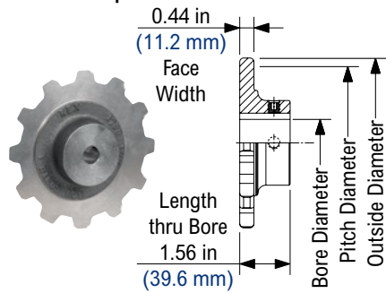
1700 Cast Iron Sprocket
