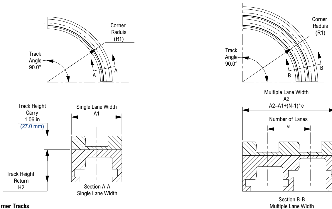
LPC1050 Corner Tracks
