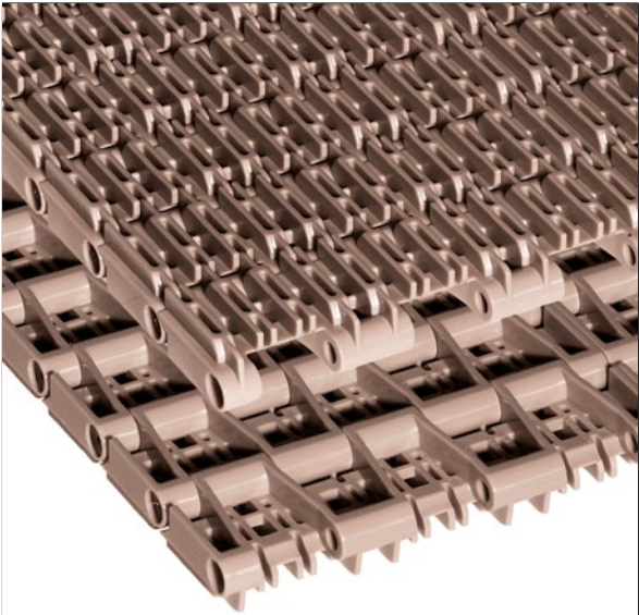
Photo shows 4707 MatTop Chain molded in Low Friction (LF) material.
