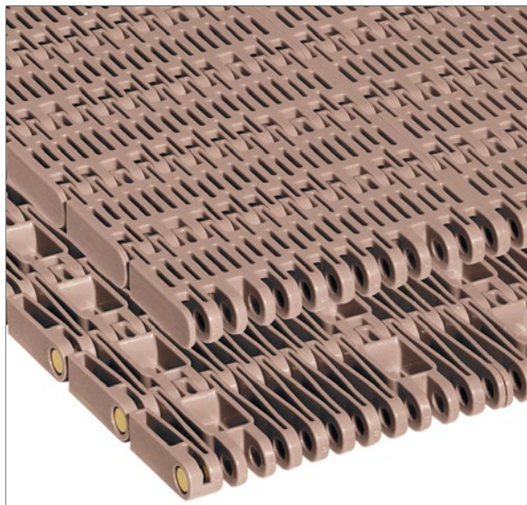
Photo shows 5996 MatTop Chain molded in Low Friction (LF) material.
